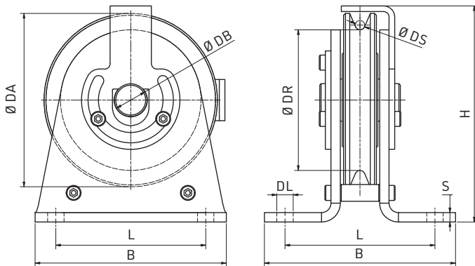
Option: Load measuring pin
