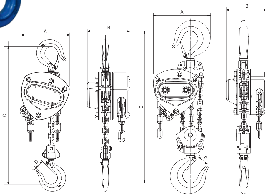
PULLMASTER-II 500-1,500 kg
