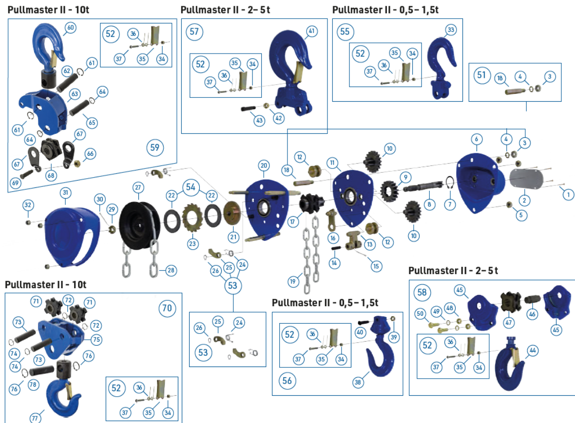
Bord 8 Reservedele PULLMASTER-II 0,5t-1,5t
