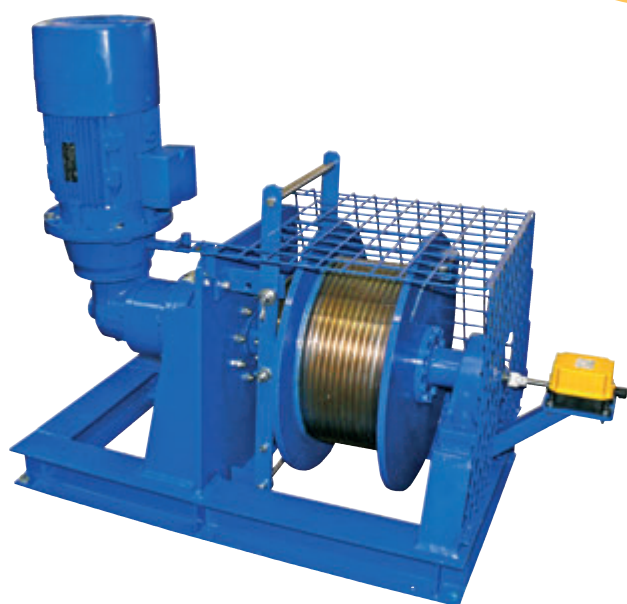
PHW 304-E with angled gear and manual freewheel clutch
